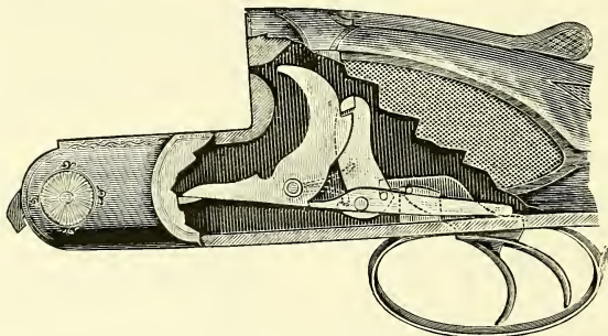
Greener's Automatic Intercepting Safety Bolt.
